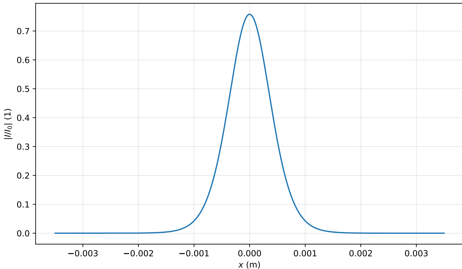
Intensity profile I(x, y = 0, z = 2.229m)/I_0 , P_{in}=0.5P_{cr} , artificial time
